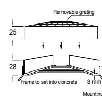
INSTALLATION EXAMPLE Stainless steel slot channel
