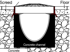
INSTALLATION EXAMPLE Stainless steel slot channel
