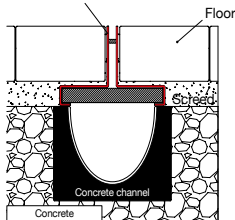
INSTALLATION EXAMPLE Stainless steel slot channel
