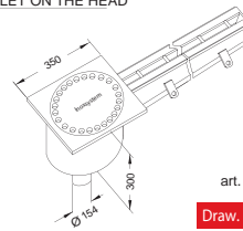
art. CFVM ..... Draw. N° 1073 - 14
