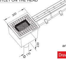
art. CFVCG ..... Draw. N° 2253 - 14
