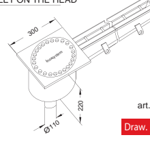
art. CFVS ..... Draw. N° 1063 - 14
